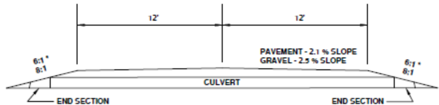
TYPICAL PRIVATE DRIVE & FIELD ENTRANCE CULVERT INSTALLATION CROSS SECTION NOT TO SCALE
